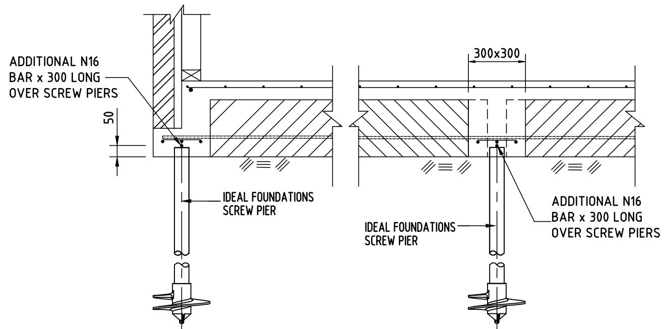
TYPICAL SCREW PIER CONNECTION DETAILS
