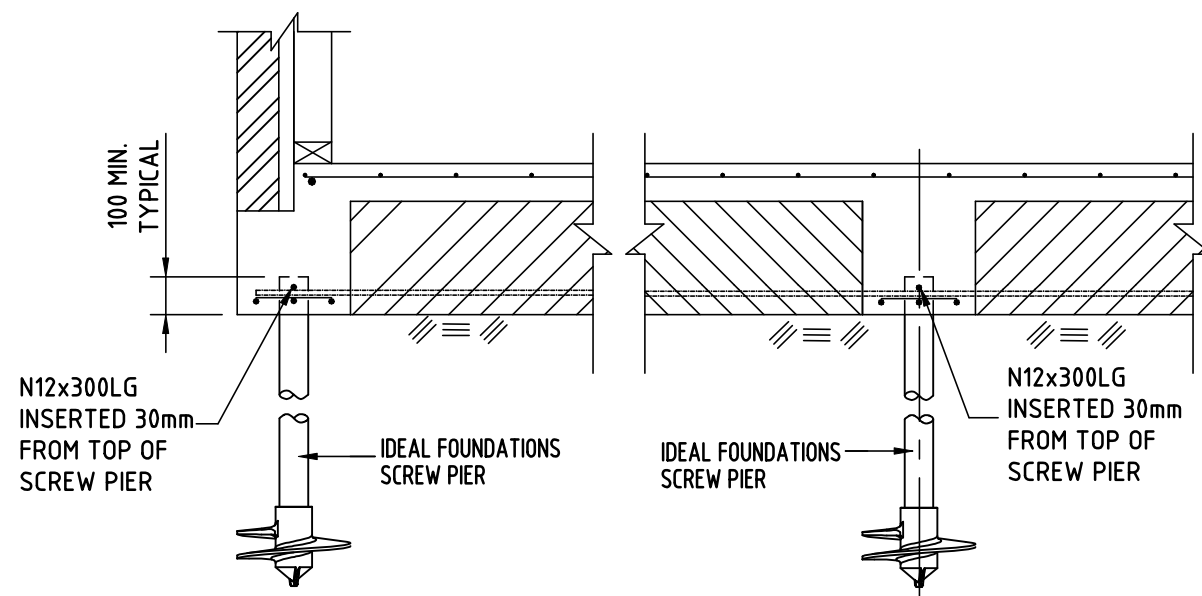
TYPICAL SCREW PIER CONNECTION DETAILS
